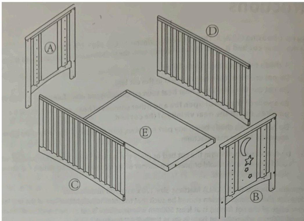
A: Left Crib End (1 pc) B: Right Crib End (1 pc) C: Front Rail (1 pc) D: Back Rail (1 pc) E: Mattress Support (1 pc)
